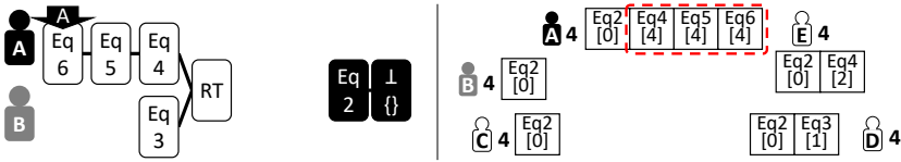
(d) ADO method invocation and multi-Paxos local log update (within A, Eq4's ballot number is updated and Eq5 and Eq6 are added locally).
