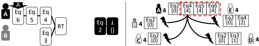
(e) ADO push and multi-Paxos phase 2 failure due to a network disconnection.
