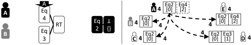
(c) ADO pull and multi-Paxos phase 1 preemption (A proposes a larger ballot number than B and finds an uncommitted log entry Eq4; Eq3 is ignored because its ballot number is smaller than that of Eq4).
